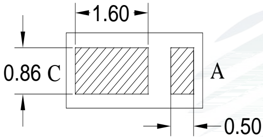
Fig. 1-4 Polarity
